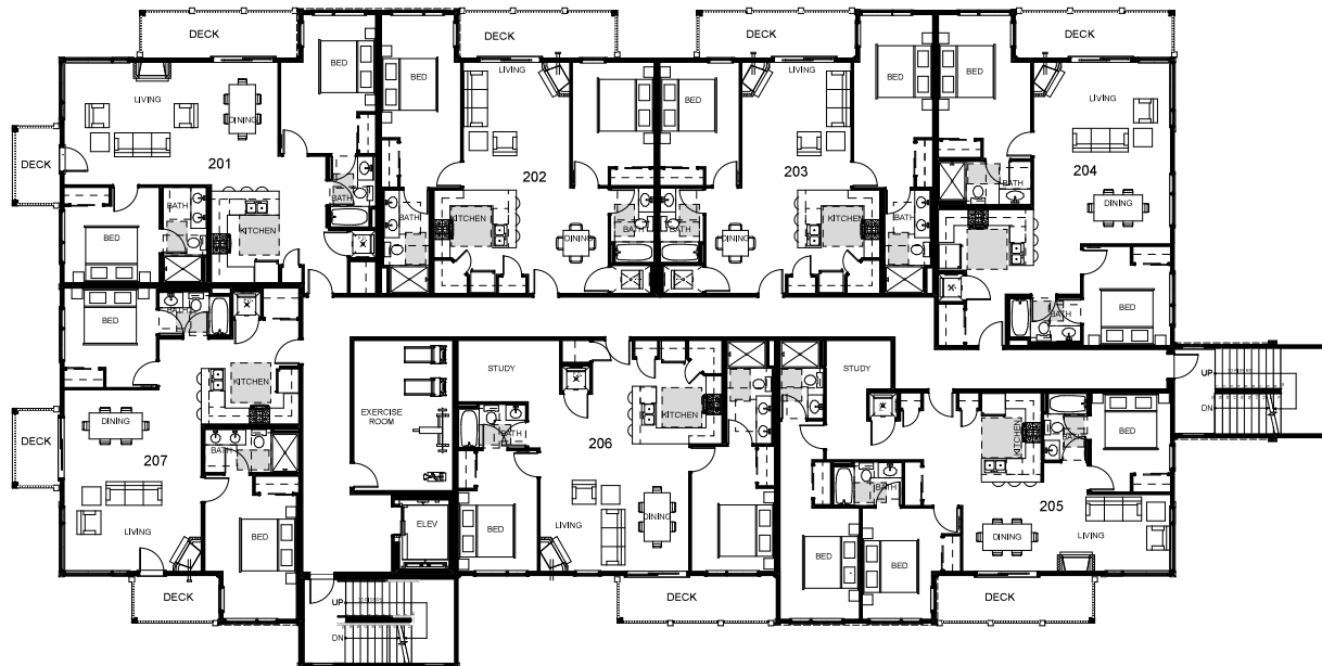
1 A-3 2ND FLOOR PRESENTATION PLAN SCALE: 1/8" = 1'-0"
