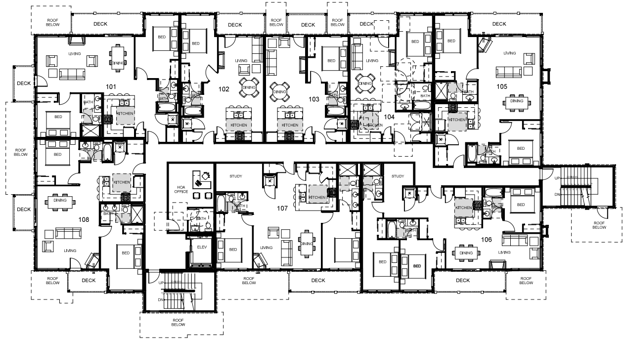
1 1ST FLOOR PRESENTATION PLAN SCALE: 1/8" = 1'-0"
